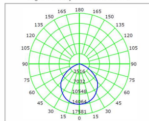
Light intensity distribution curve
