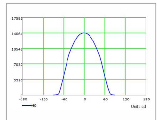
Emission cone luminous flux
