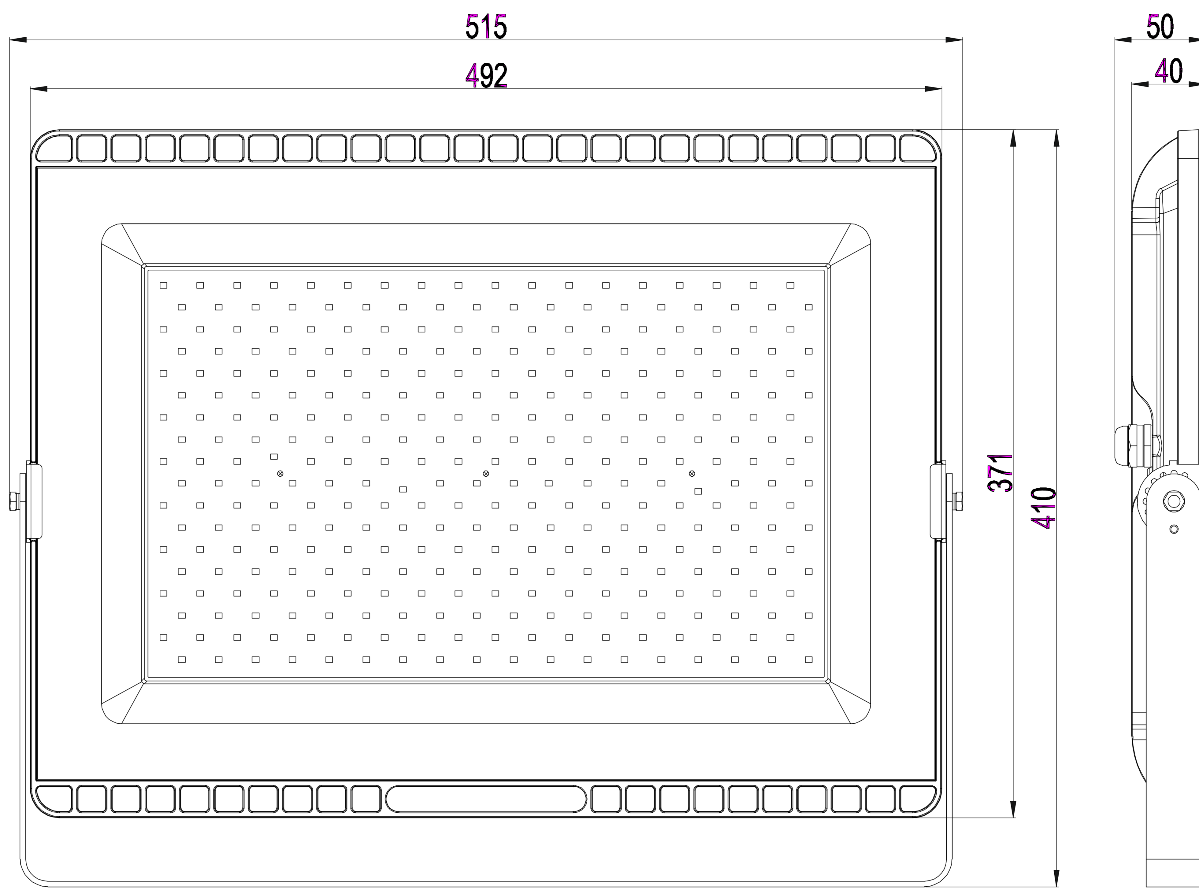
FR-PL300Mx_Dimensions
