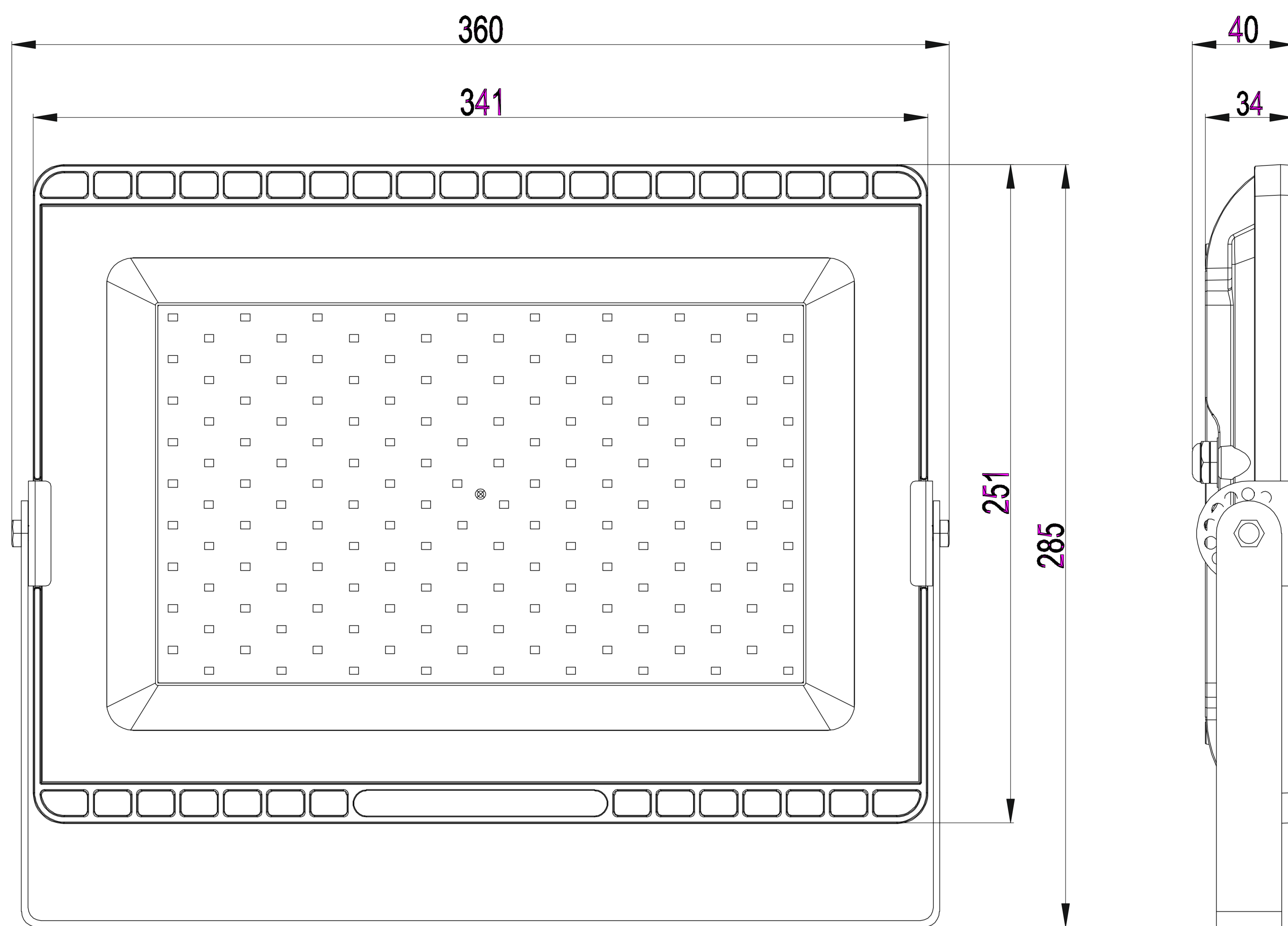
FR-PL150Mx_Dimensions
